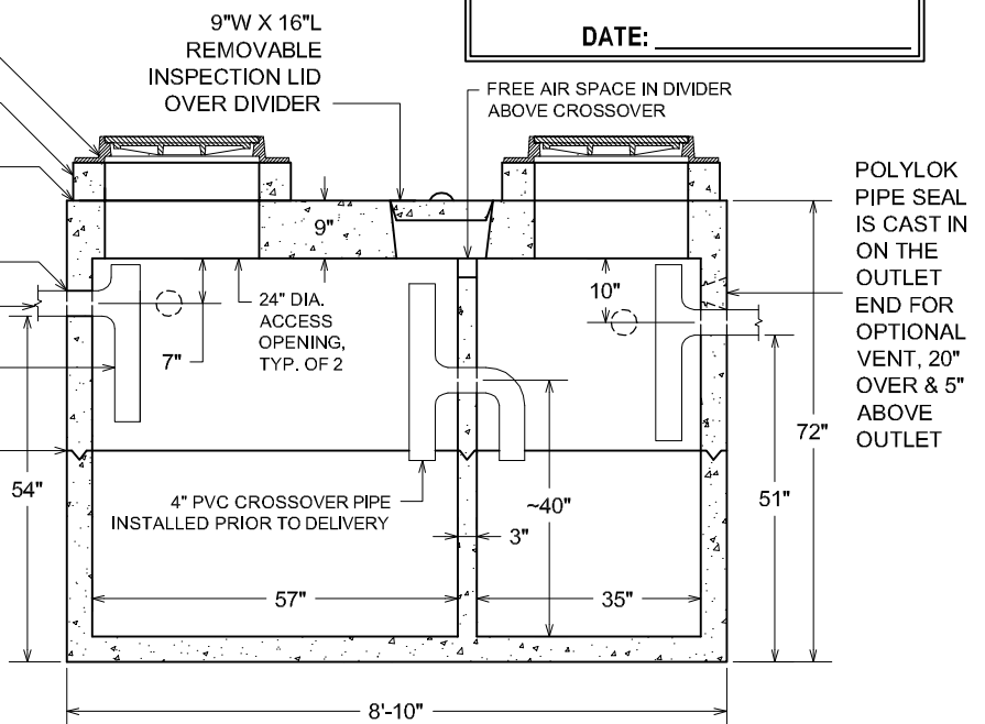
SECTION VIEW
