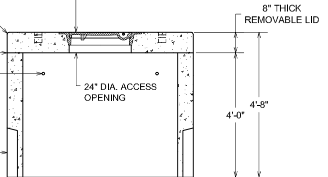
SECTION VIEW
