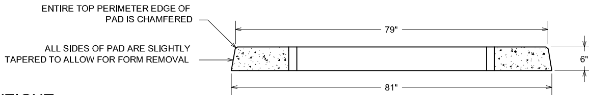
SECTION VIEW
