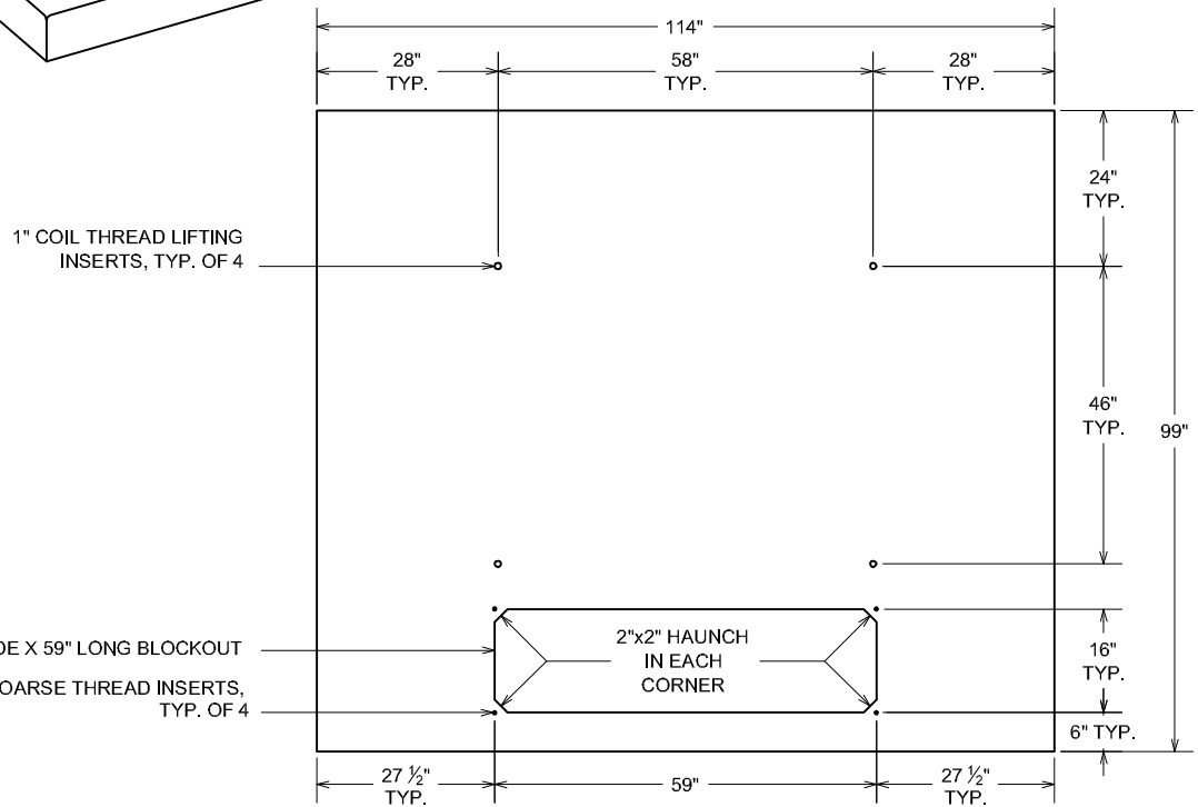
PLAN VIEW
