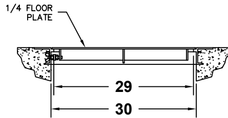
SECTION VIEW FRONT
