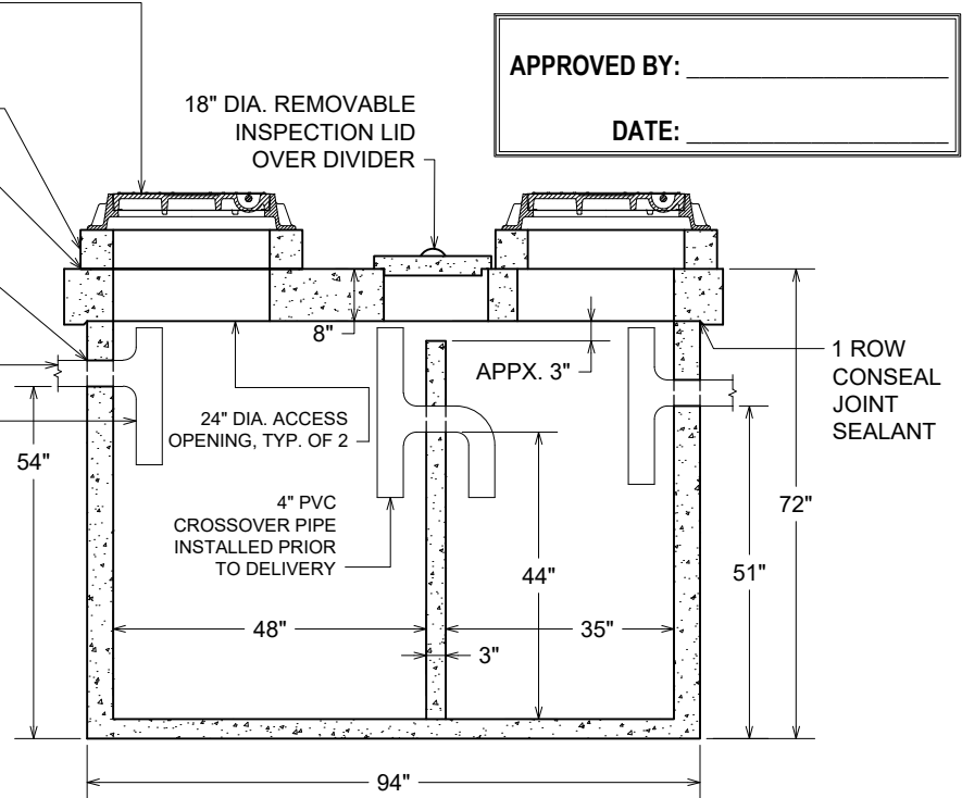
SECTION VIEW
