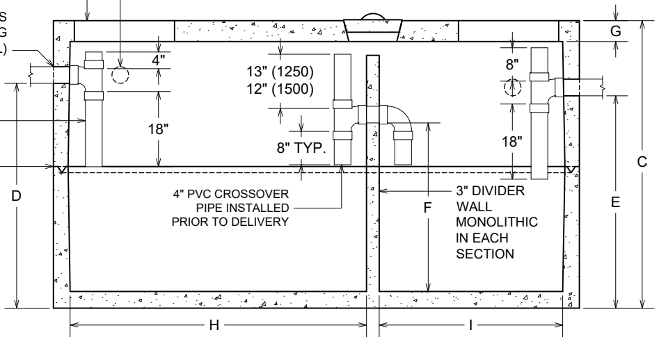
SECTION VIEW
