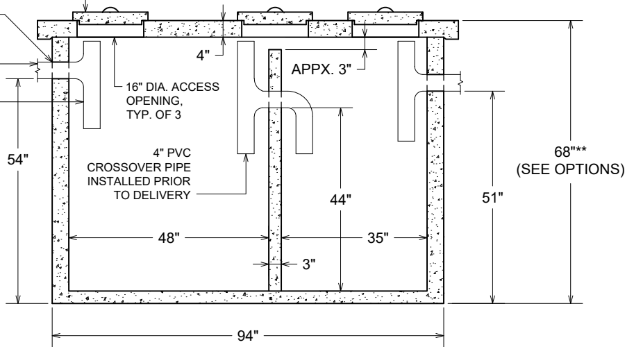
SECTION VIEW
