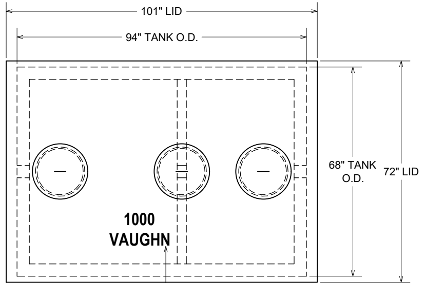
PLAN VIEW
