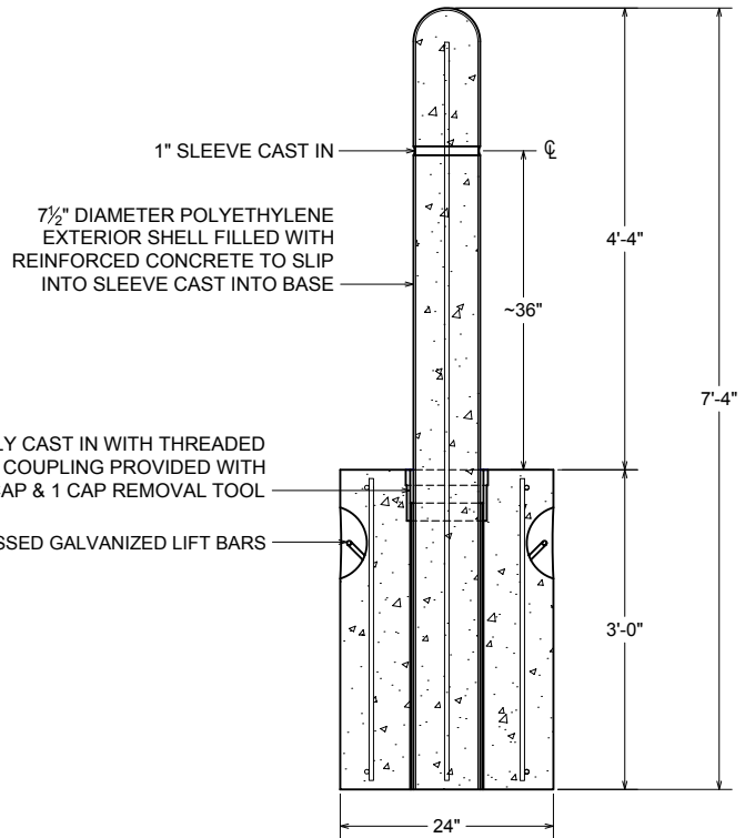
SECTION VIEW
