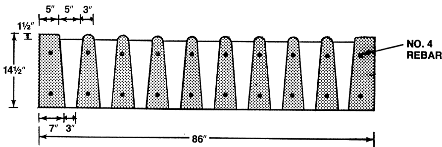
END SECTION VIEW
