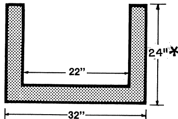
Concrete 4000 P.S.I. (Minimum) Reinforced with Rebar and Wire Mesh
